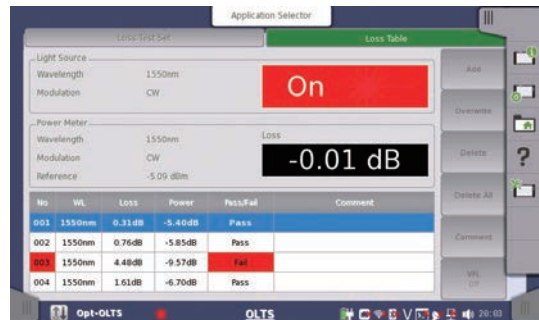
OLTS Measurement Loss Table Screen
