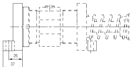
Clevis Mount Set(LA64-CMS)
