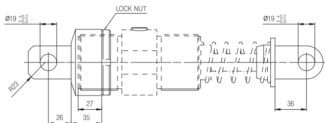
Clevis Mount Set(LA64-CMS)
