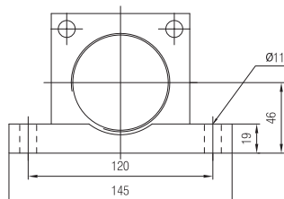
Foot Mount(LA64-FM)
