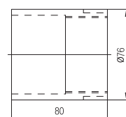
Stop Collar(LA64-SC)
