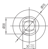
Cylinder Clevis(LA64-CC)
